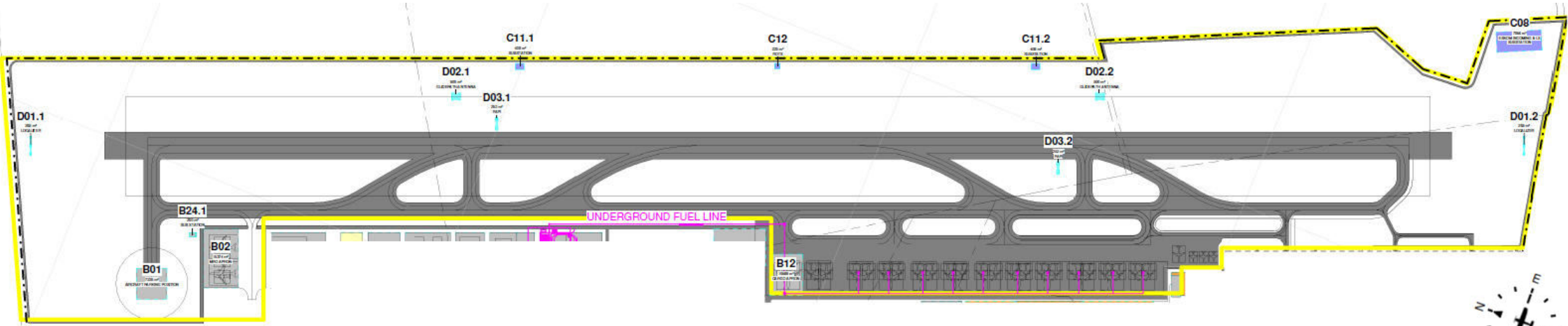
Proposed layout of main runway 01-19, from drawing 2024-3297 404, Rev 14, dated 2024-08-20
