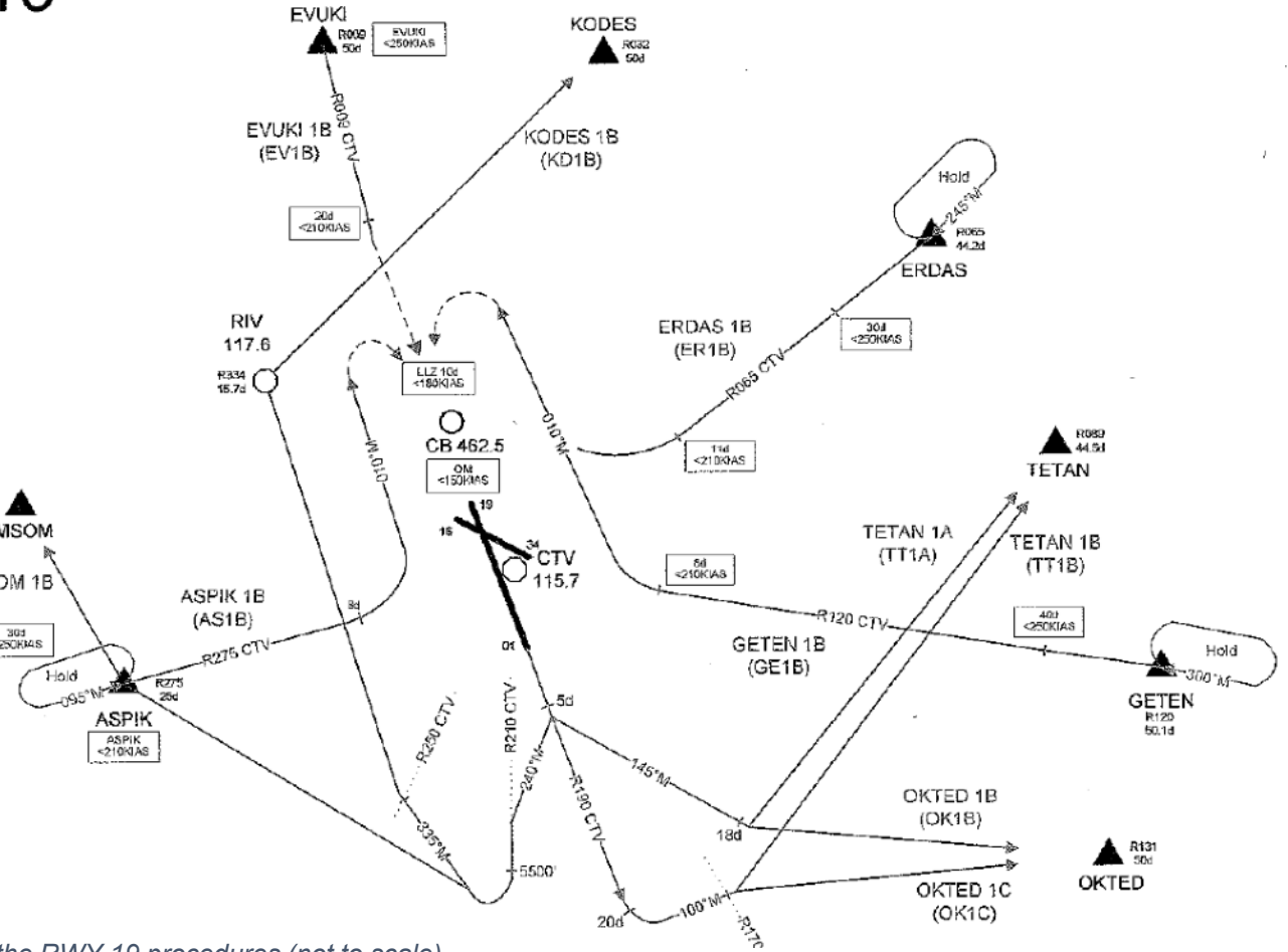
Schematic overview of the RWY 19 procedures (not to scale).
