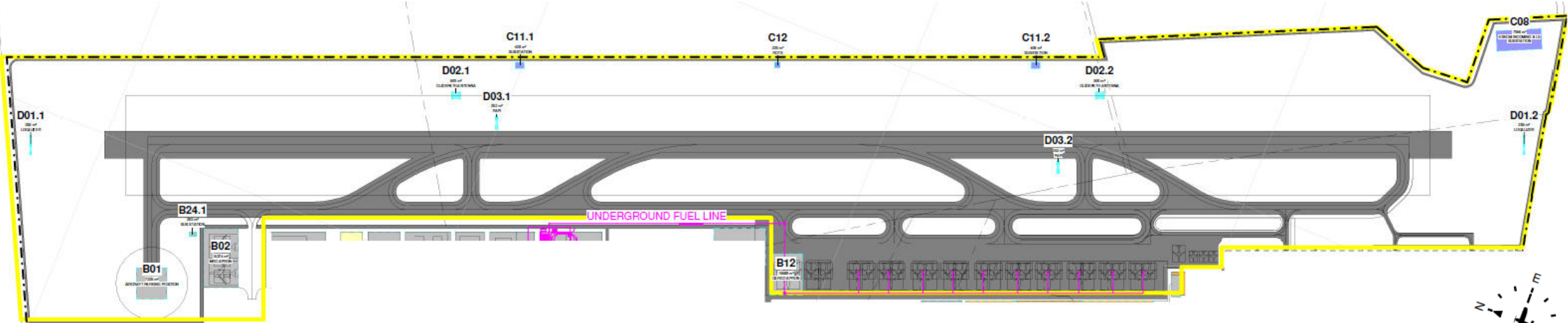
Proposed layout of main runway 01-19, from drawing 2024-3297 404, Rev 14, dated 2024-08-20
