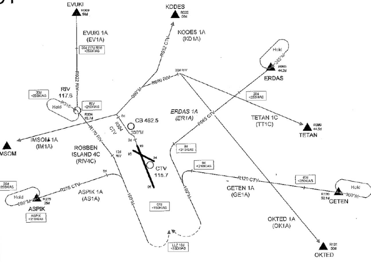
Schematic overview of the RWY 01 procedures (not to scale).
