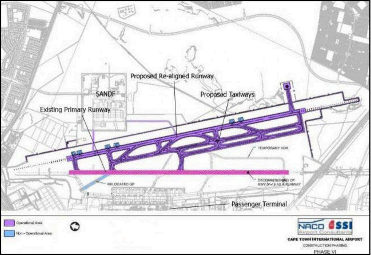
Proposed layout of the New Realigned Runway at Cape Town International Airport
