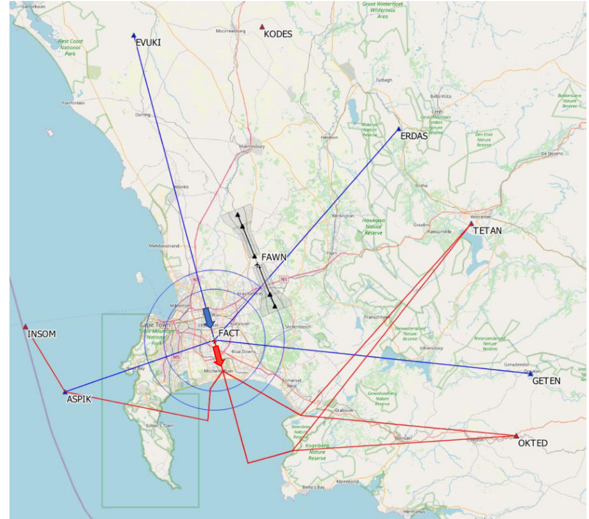
Schematic overview of the procedures for RWY 19. Arrivals in blue and departures in red
