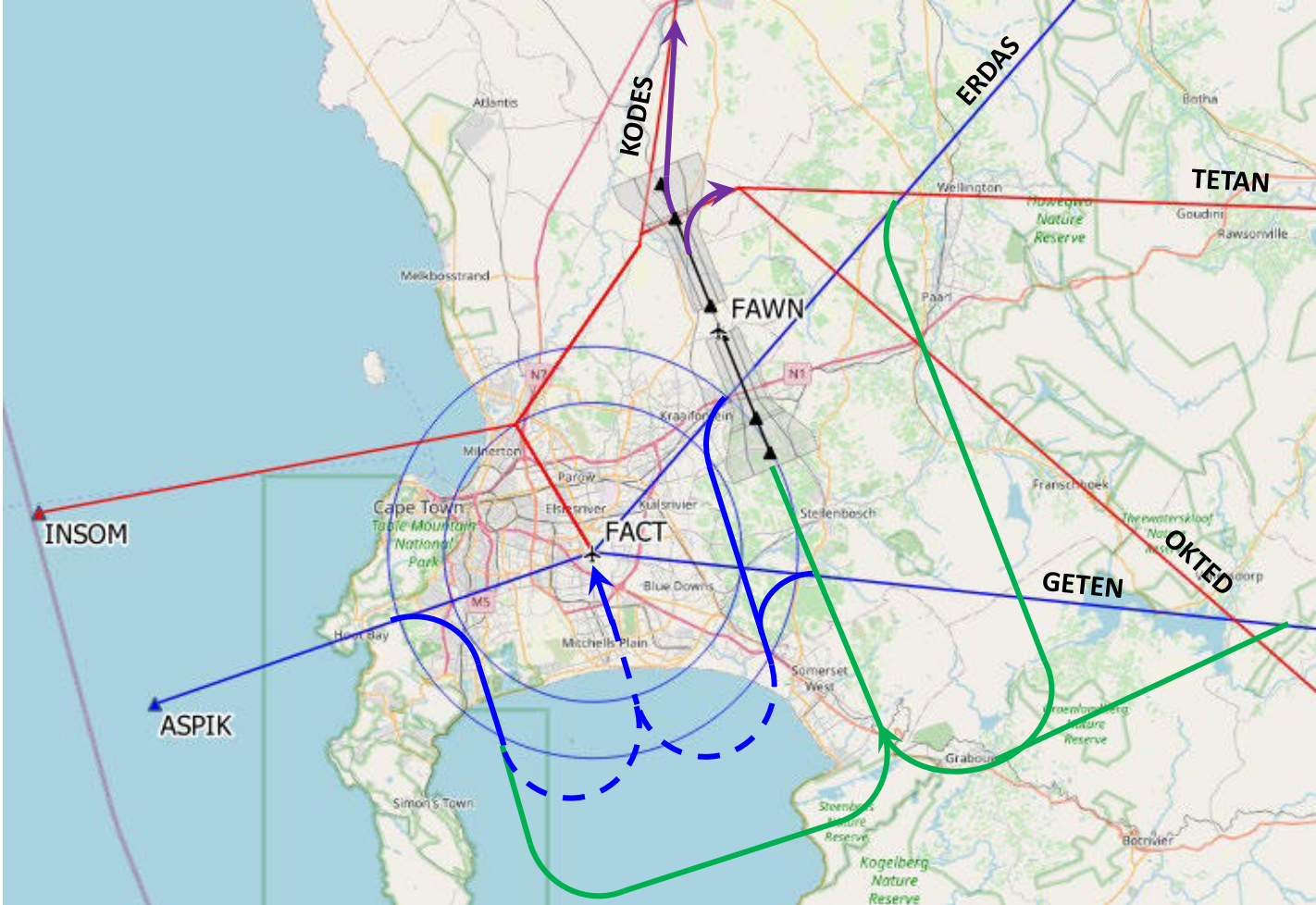
Schematic overview of potential merger of traffic flows in a northern operation
