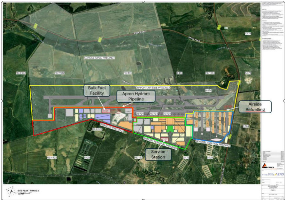
Figure 3-1: Site layout
