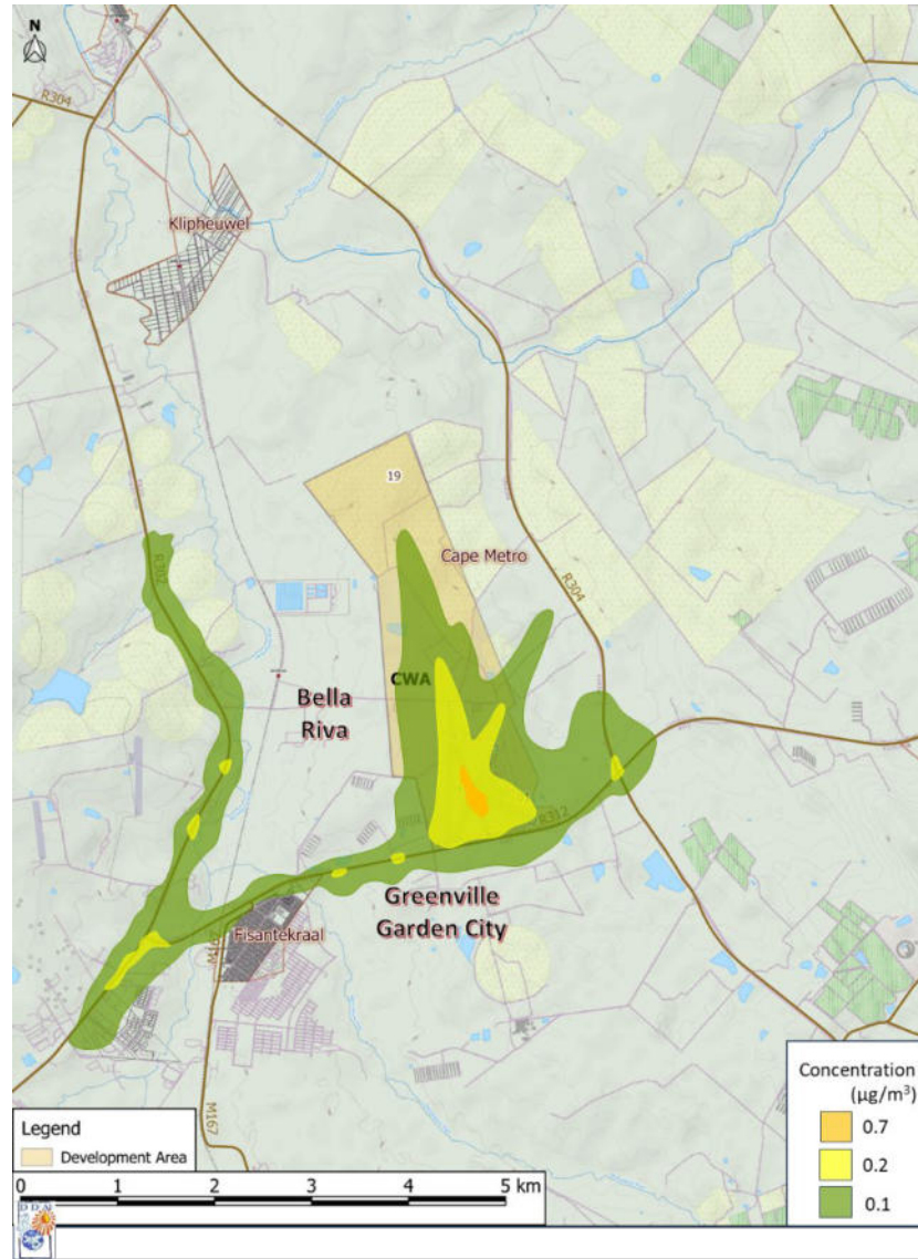
Figure 5-9. Scenario 1: PM 2.5 24-hr Maximum Concentrations (Guideline 60 µg/m 3 )
