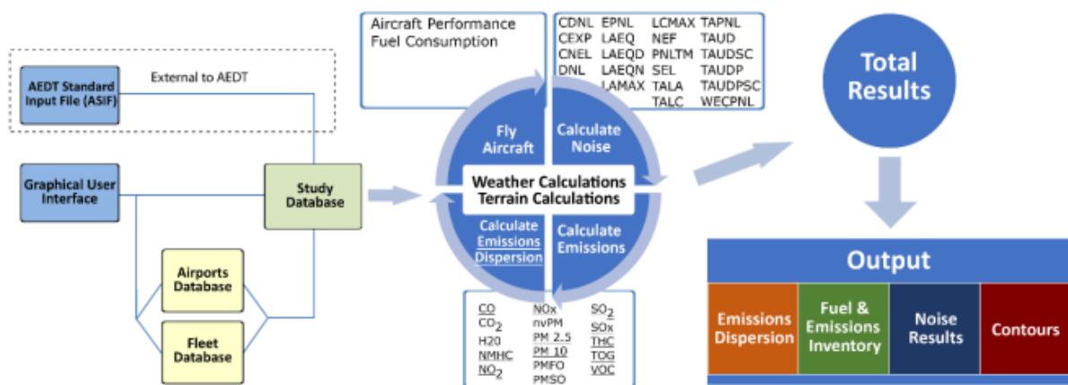
Figure 5-1. AEDT System Architecture
