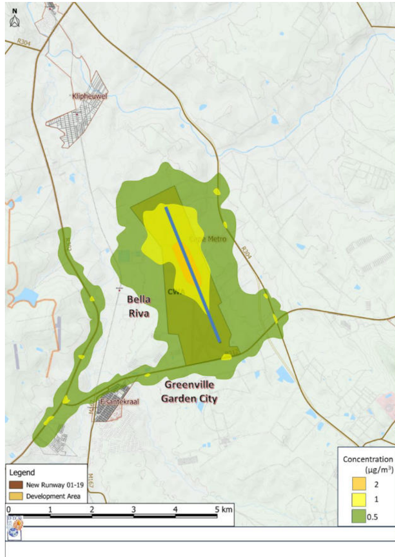
Figure 5-16. Scenario 3: PM 2.5 24-hr Maximum Concentrations (Guideline 40 µg/m 3 )
