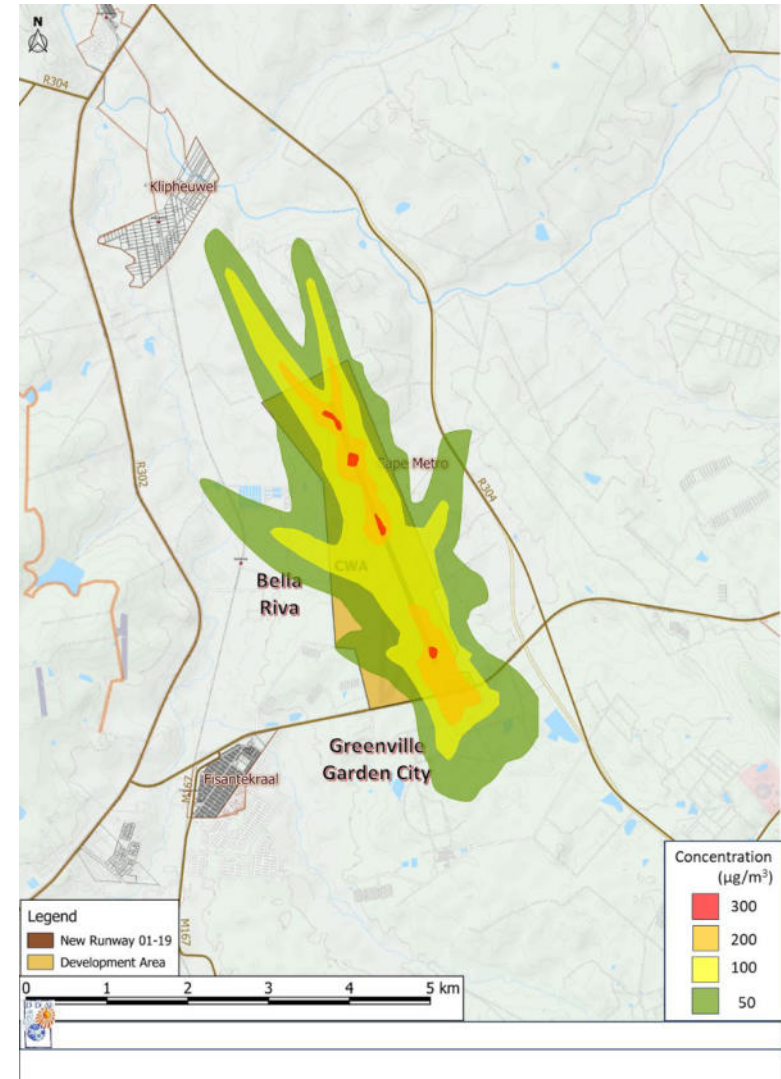
Figure 5-11. Scenario 3: NO 2 1-hr Maximum Concentrations (Guideline 200 µg/m 3 )
