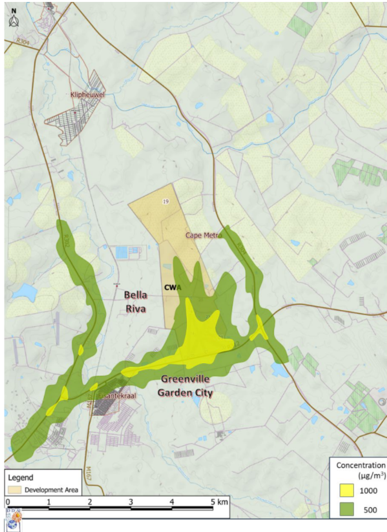
Figure 5-3. Scenario 1: CO 1-hr Maximum Concentrations (Guideline 30,000 \mu\text{g}/\text{m}^3 )
