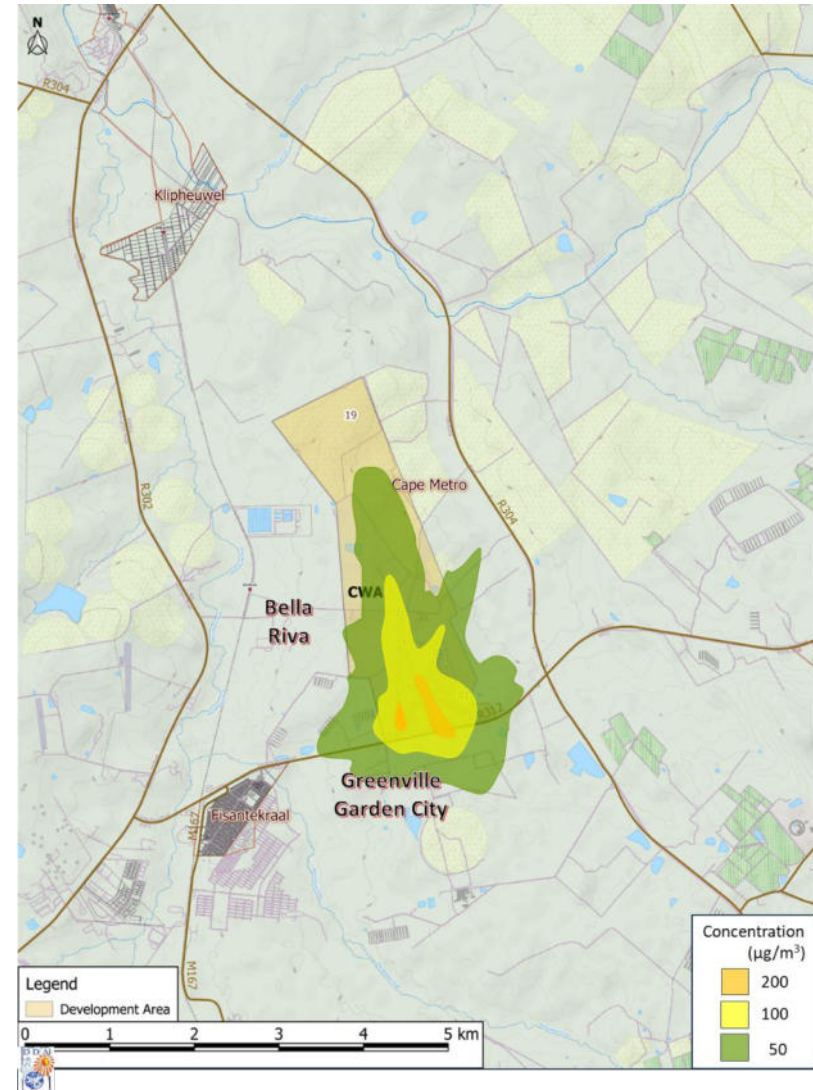
Figure 5-4. Scenario 1: NO 2 1-hr Maximum Concentrations (Guideline value: 200 \mu\text{g}/\text{m}^3 )
