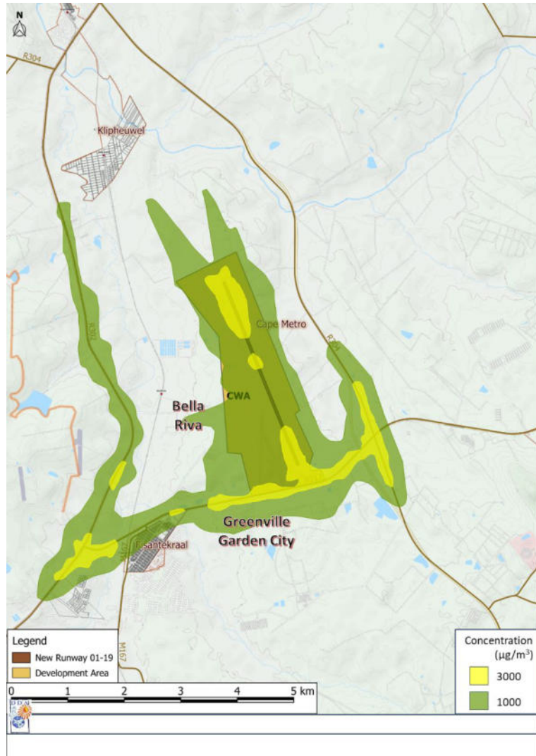
Figure 5-10. Scenario 3: CO 1-hr Maximum Concentrations (Guideline 30,000 µg/m 3 )
