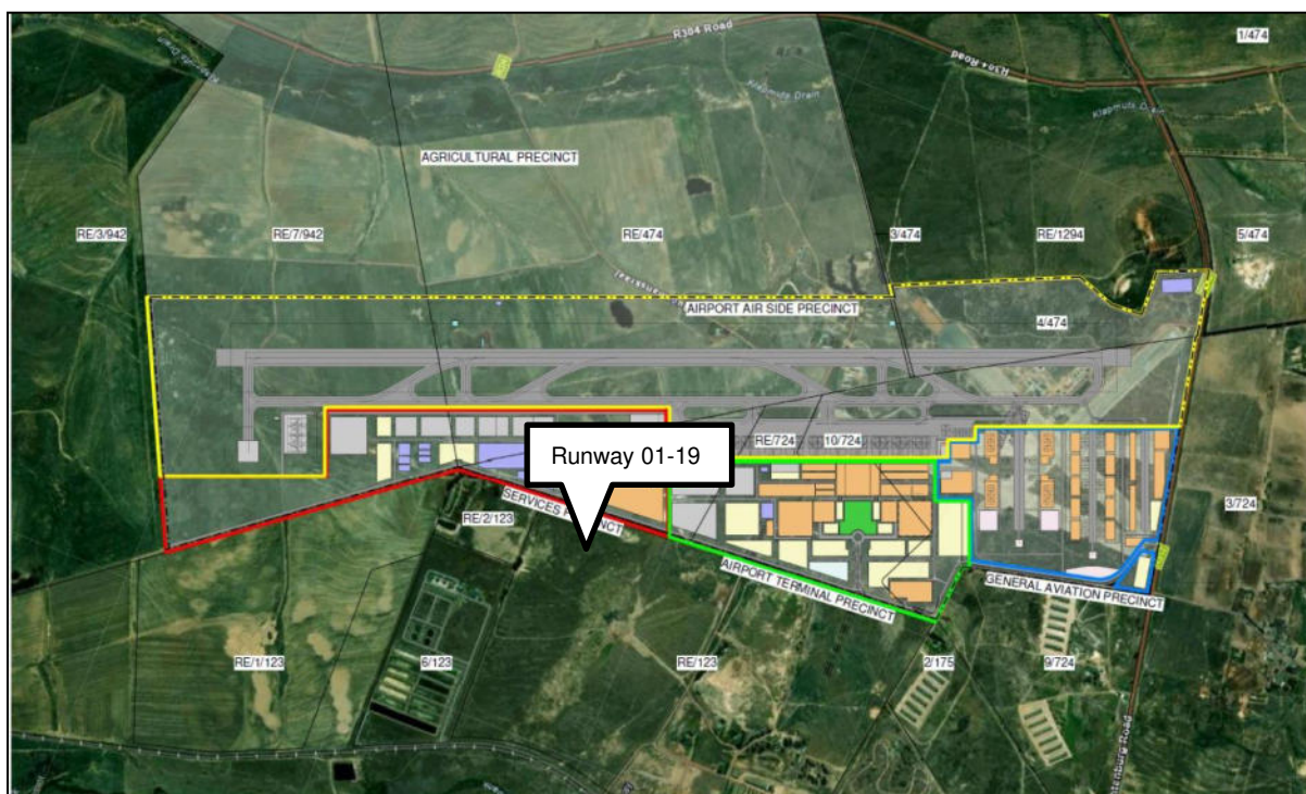
Figure 5: Proposed layout of the CWA development during Phase 2 of the preferred alternative.
